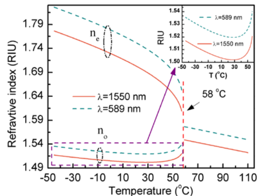
Fig. 1. Temperature-dependent refractive indices of E7 at \lambda=589\text{ nm} and \lambda=1550\text{ nm} , respectively. The inset shows the enlarged temperature characteristics of the refractive indices of LC, i.e., E7.
