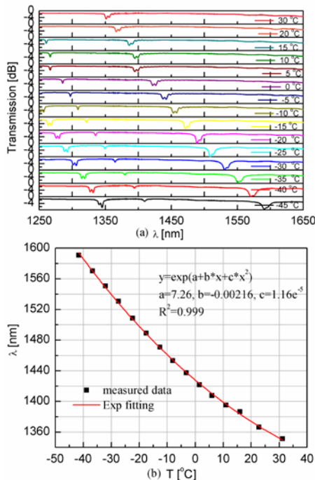
Fig. 5. (a) The transmission spectra of the SLPCPF corresponding to variations in temperature from -45 °C to 30 °C; (b) Temperature sensitivity of \lambda_{res1} .
