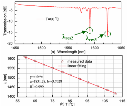
Fig. 7. (a) The transmission spectra of the SLPCPF corresponding to variations in temperature from 59 °C to 110 °C; (b) Temperature sensitivity of \lambda_{res2} .
