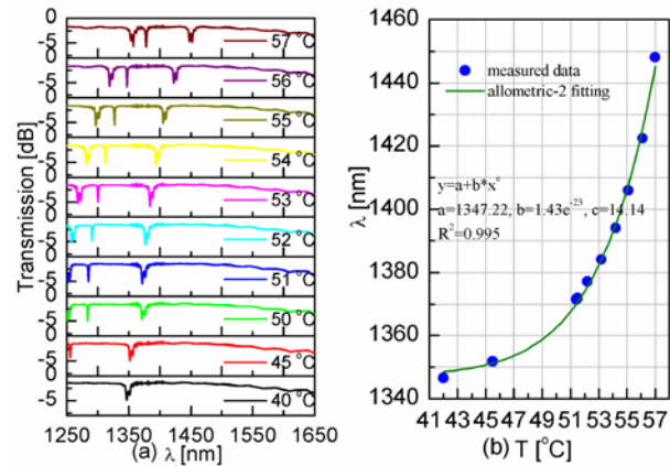
Fig. 6. (a) The transmission spectra of the SLPCPF corresponding to variations in temperature from 40 °C to 57 °C; (b) Temperature sensitivity of \lambda_{res1} .
