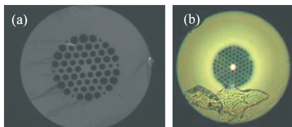
Fig. 2. (a) Cross section images of (a) pure-silica PCF (IPHT-84b1a) and Ge-doped PCF (IPHT-282b5).
