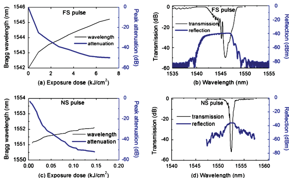
Fig. 5. FBGs written in Ge-doped PCFs after H_2 -loading with (a), (b) a FS laser (FS pulse) and (c), (d) an excimer laser (NS pulse), (a) and (c) development of Bragg wavelength and peak attenuation with increasing exposure dose, (b) and (d) transmission and reflection spectra of the FBGs.
