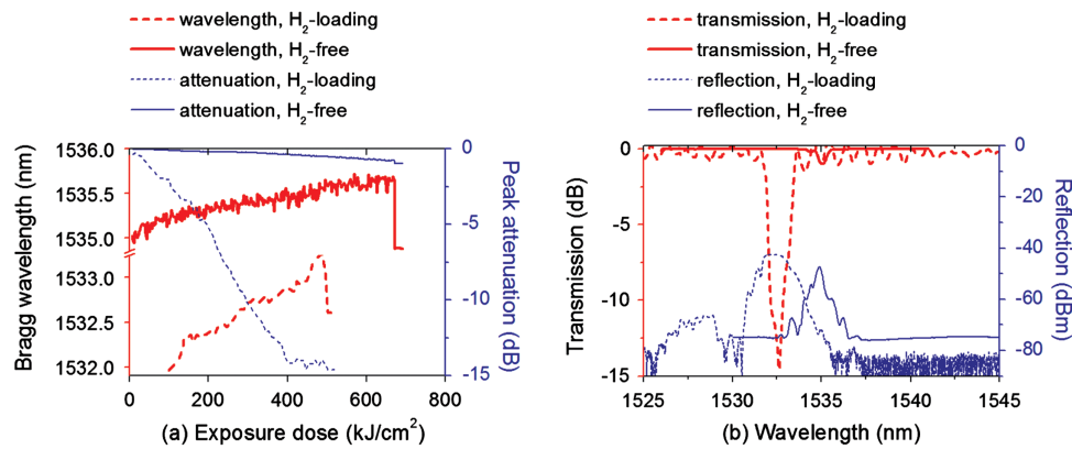
Fig. 3. FBGs written in pure-silica PCFs before/after H 2 -loading with a FS laser, (a) development of Bragg wavelength and peak attenuation with increasing exposure dose, (b) transmission and reflection spectra of the FBGs.
