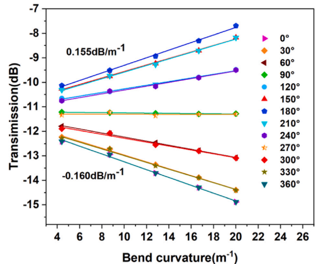
Fig. 7. The relationship between resonance intensity and bending curvature at various bending directions.
