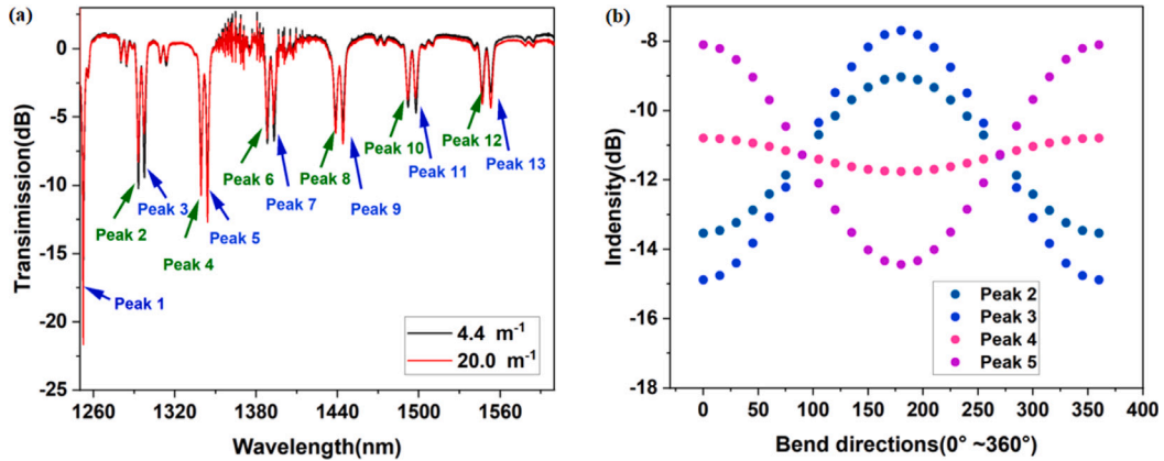
Fig. 4. Transmission spectra of the Ex-TFG sensor under two different bending curvatures: 4.4 \text{ m}^{-1} and 20.0 \text{ m}^{-1} , with a fixed bending direction. (b) Intensity variations of peaks 2, 3, 4, and 5 as a function of bending direction at a fixed curvature of 20.0 \text{ m}^{-1} .
