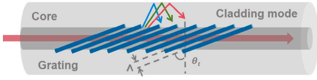
Fig. 1. Schematic structure of Ex-TFG.
