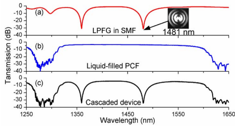
Fig. 2. Transmission spectra of (a) the LPFG, inset: the near mode field pattern of LP 14 cladding mode at 1481 nm, (b) the liquid-filled PCF, and (c) the cascaded LPFG and liquid-filled PCF device.
