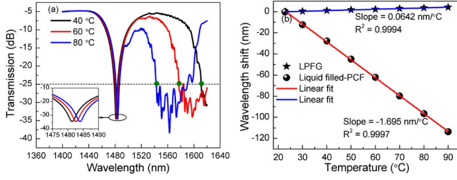
Fig. 3. (a) Transmission spectra of the proposed device at temperatures of 40, 60, and 80 °C, inset: enlarged resonant dip of the LPFG, (b) wavelength shift of the LPFG and the liquid-filled PCF at different temperature.
