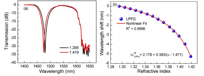
Fig. 4. (a) Transmission spectra of the proposed device immersed in the liquids with a RI of 1.295 and 1.419, (b) resonant wavelength shift of the LPFG at different surrounding RIs.
