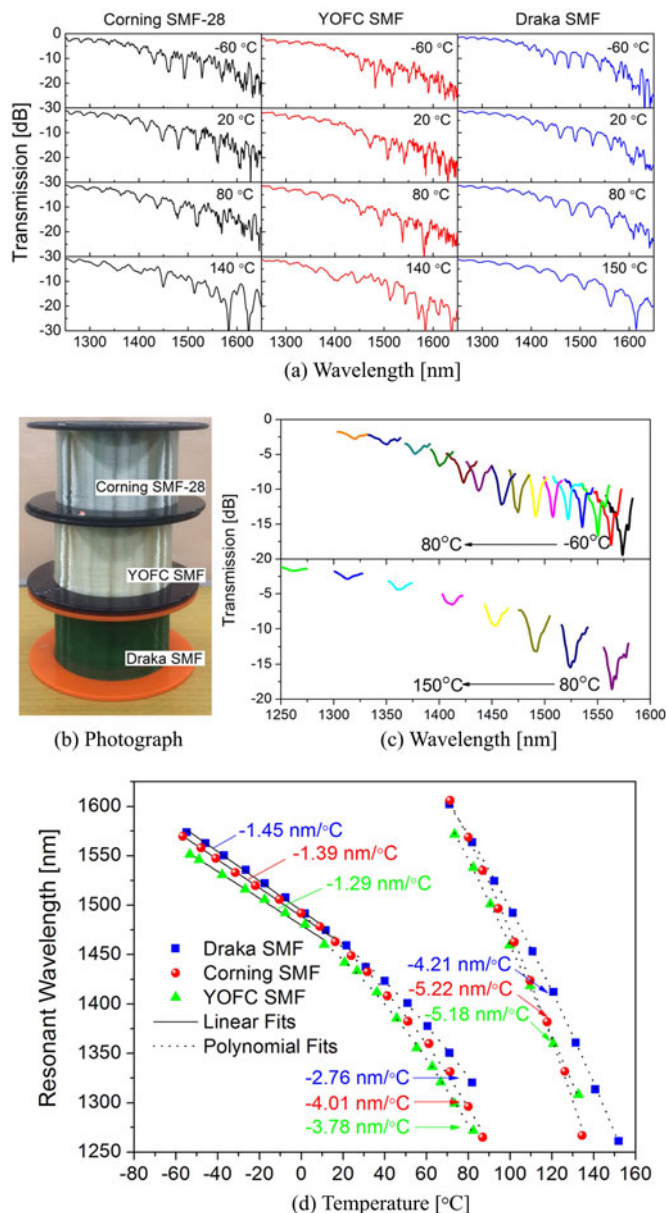
Fig. 5. (a) The transmission spectra of the three types of coated-SMF loops (Corning SMF-28, YOFC SMF, Draka SMF, R = 5 mm) at typical temperatures of -60 , 20 , 80 , 140 and 150 °C; (b) The photograph of the three types of SMFs; (c) Resonant wavelength evolution of the Draka-SMF loop with a step of 10 °C (upper: evolution of the transmission dip around 1570 nm at the initial temperature of -60 °C, lower: evolution of the transmission dip around 1570 nm at the initial temperature of 80 °C); (d) The temperature response of the three types of coated-SMF loop sensors.
